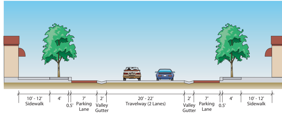
SECTION WITH ON-STREET PARKING
